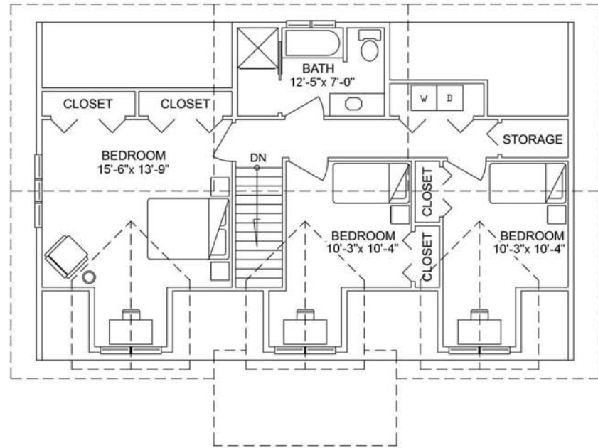
UPPER FLOOR PLAN 855 sq. ft. (79.45 sq. m.)
