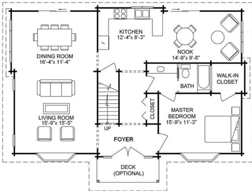
MAIN FLOOR PLAN 1243 sq. ft. (115.47 sq. m.)
